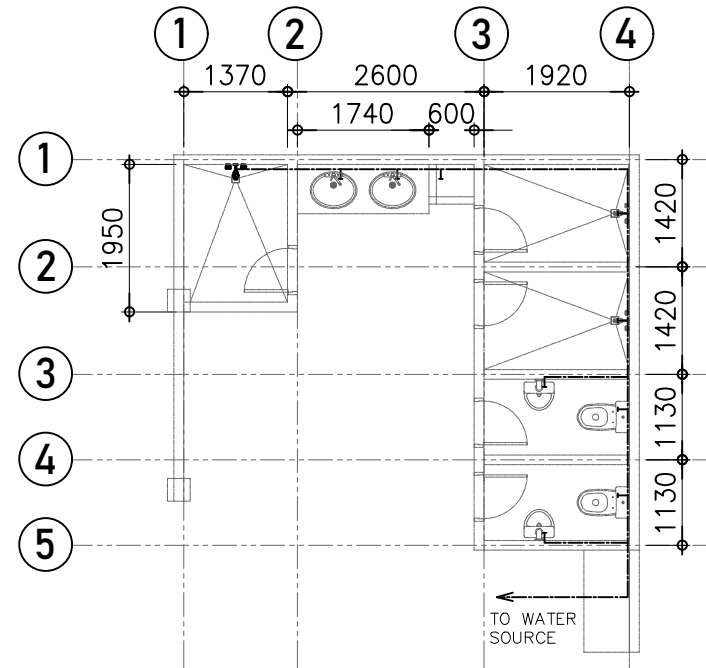
APARTMENT WATERLINE LAYOUT SCALE 1:100
