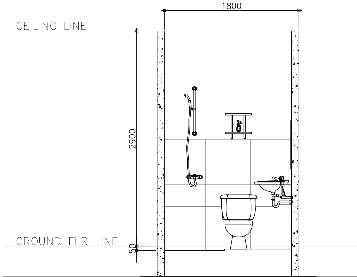
DORM T&B ELEVATION SCALE NTS
