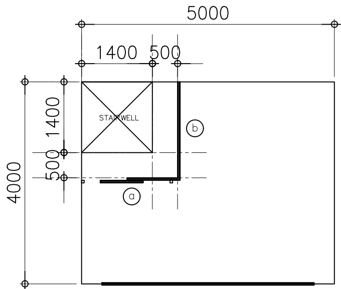
COTTAGE ATTIC GLASS PARTITION PLAN
