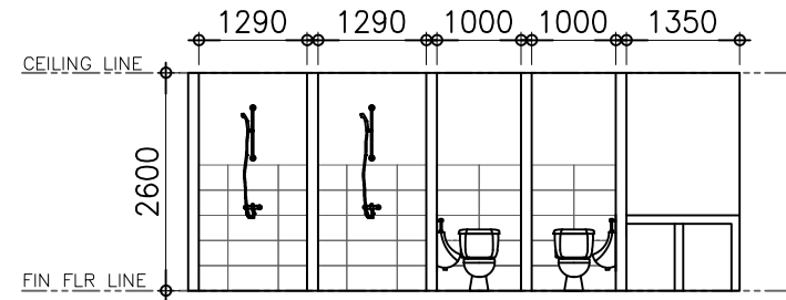
SECTION THRU S-2 SCALE 1:100
