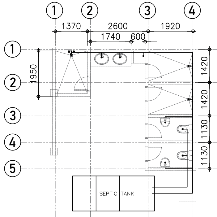
APARTMENT PLUMBING LAYOUT SCALE 1:100
