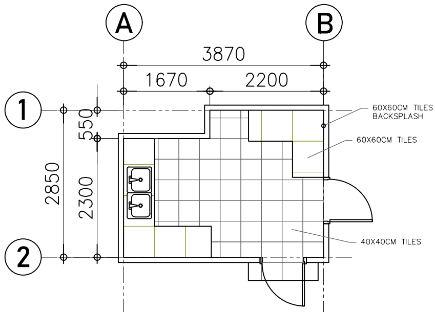
COTTAGE KITCHEN TILE LAYOUT
