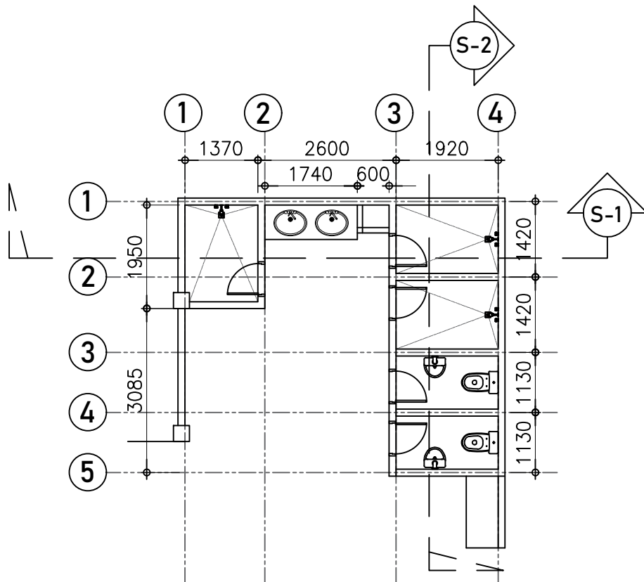
APARTMENT CR FLOOR PLAN SCALE 1:100
