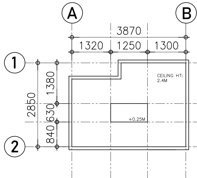
COTTAGE KITCHEN CEILING PLAN
