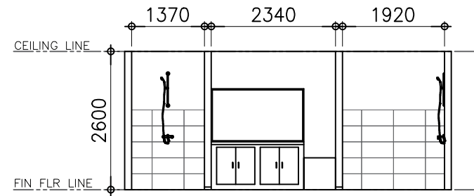
SECTION THRU S-1 SCALE 1:100
